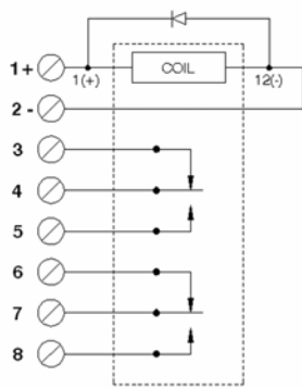
WIRING SCHEMATIC (per Relay)
